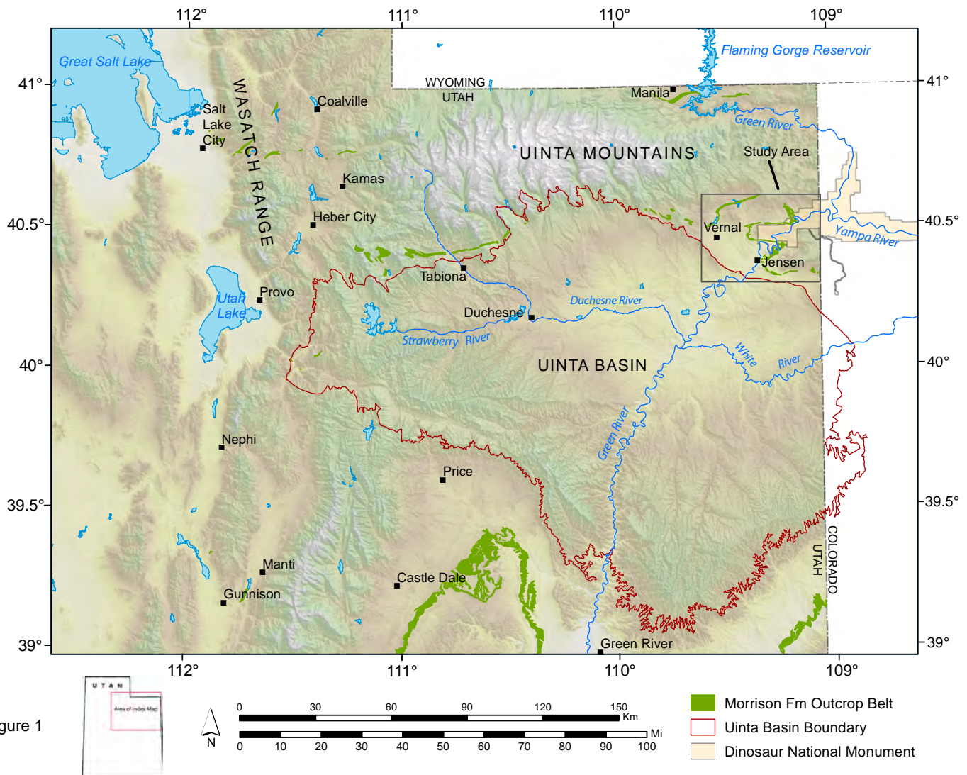
Figure 1. Regional map showing the Morrison Formation study area in the eastern Uinta Mountains of northeastern Utah, USA. Morrison outcrop locations from Hintze and others (2000).
