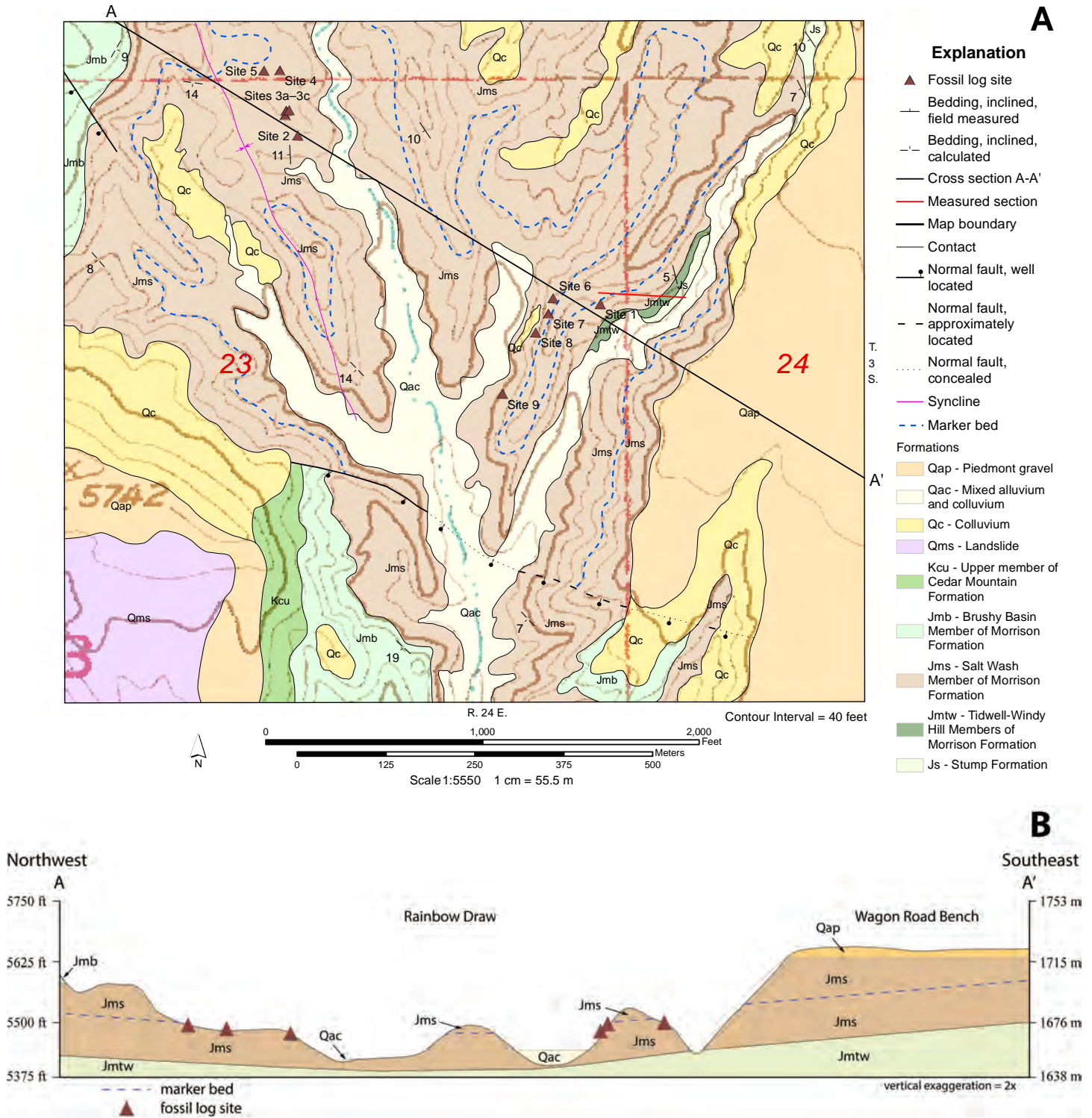
Figure 5. (A) Geologic map and (B) cross section of the Rainbow Draw area fossil log sites. The Morrison Formation overlies the Stump Formation and underlies the Cedar Mountain Formation in Rainbow Draw. In the mapped area, the Morrison includes the Windy Hill, Tidwell, Salt Wash, and Brushy Basin Members. The fossil log sites are concentrated in two groups on separate ridges. Both groups of logs occur in light-colored, fine-grained sandstone and siltstone below a mostly reddish-colored siltstone that was used as a marker bed (blue dashed line).
